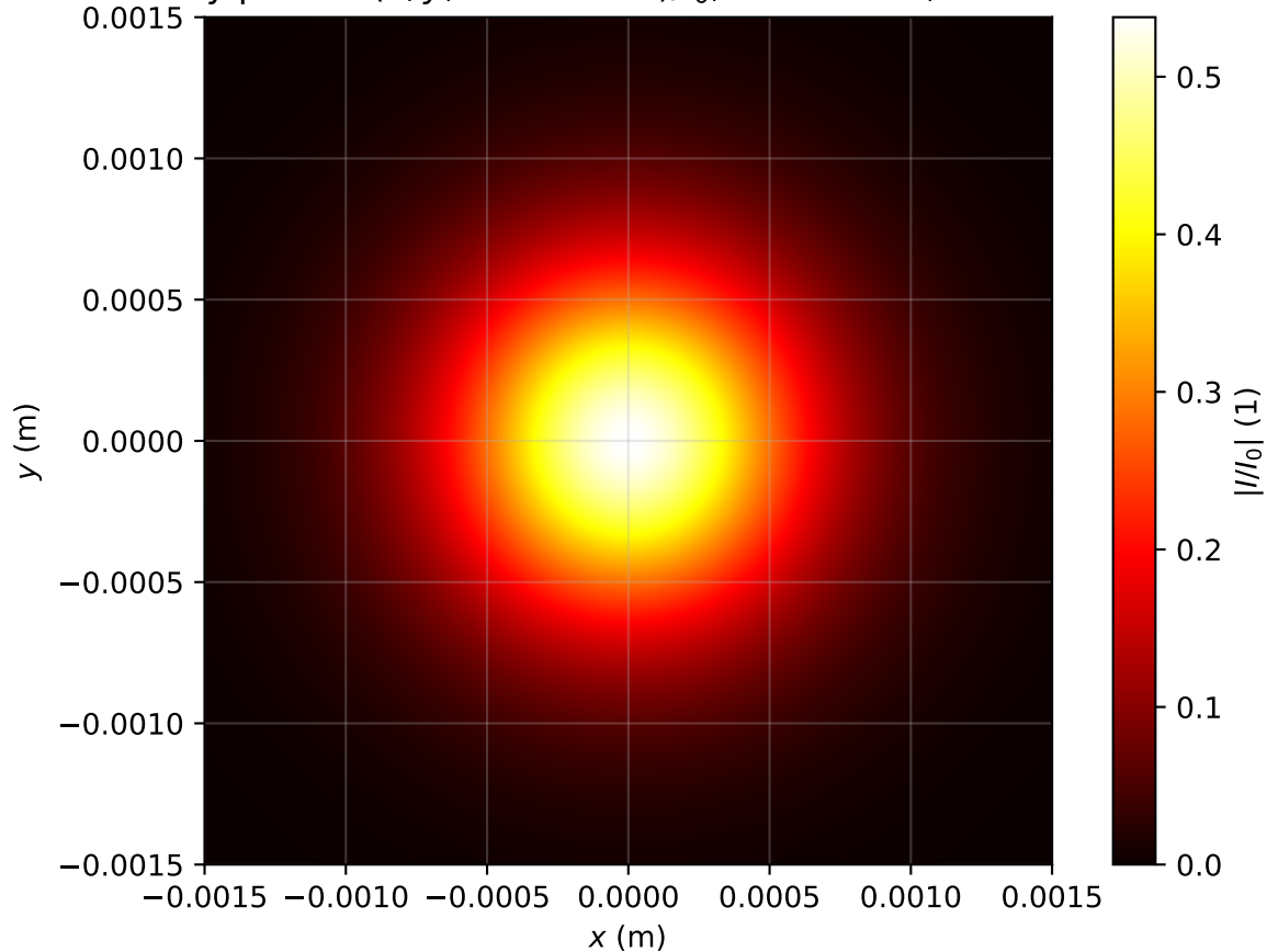
Intensity profile I(x, y, z = 3.662m)/I_0 , \text{Pin}=0.6\text{Pcr} , artificial time
